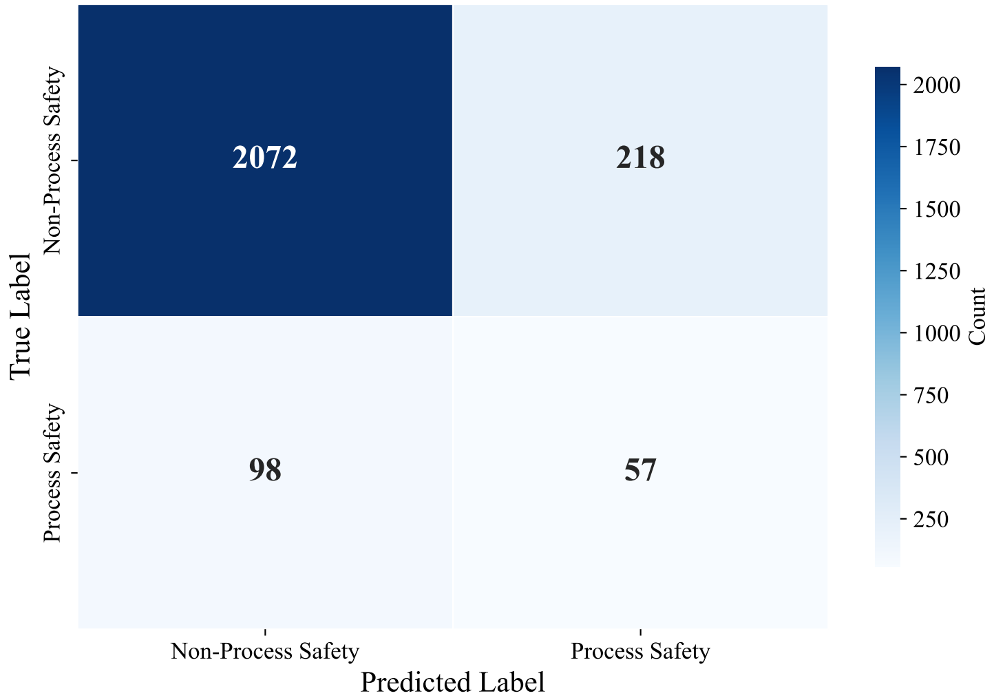
Confusion Matrix — SWEDISH_MANUAL (efederici/e5-base-multilingual-4096, XGBoost_Optimized)
