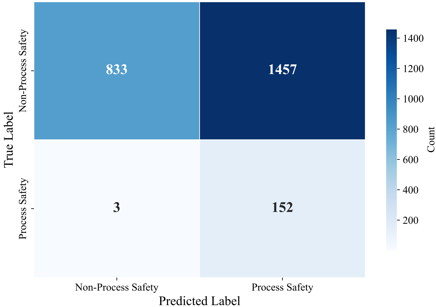
Confusion Matrix — SWEDISH_MANUAL (upskyy/bge-m3-korean, Random_Forest_Optimized)
