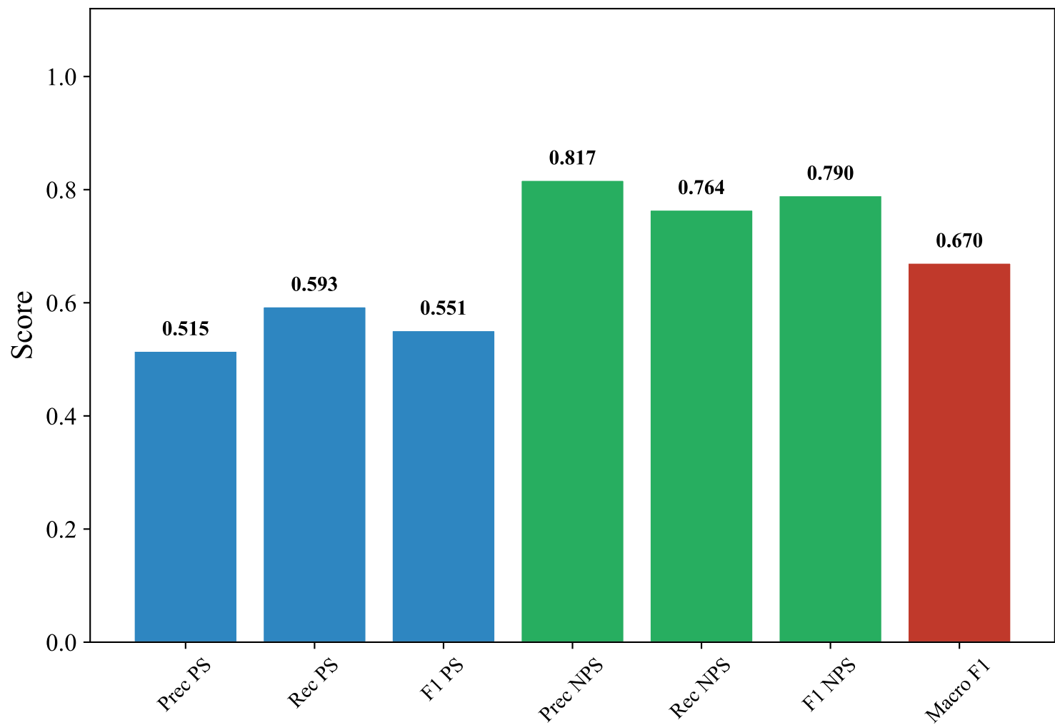
Classification Metrics — DUTCH_MANUAL (efederici/e5-base-multilingual-4096, SVM)
