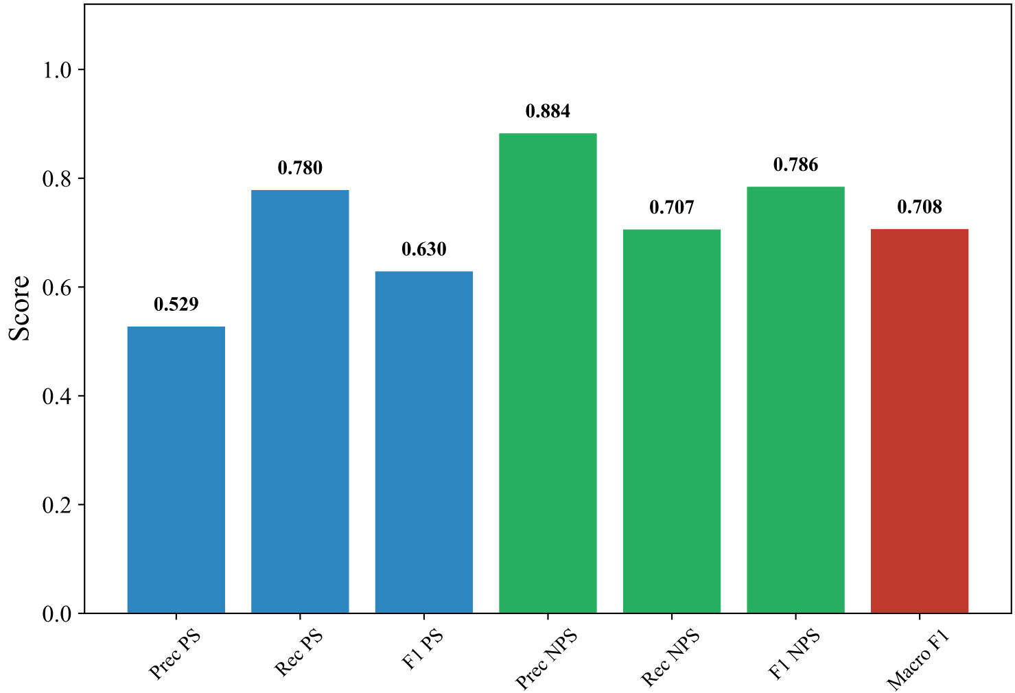
Classification Metrics — DUTCH_MANUAL (efederici/e5-base-multilingual-4096, XGBoost)
