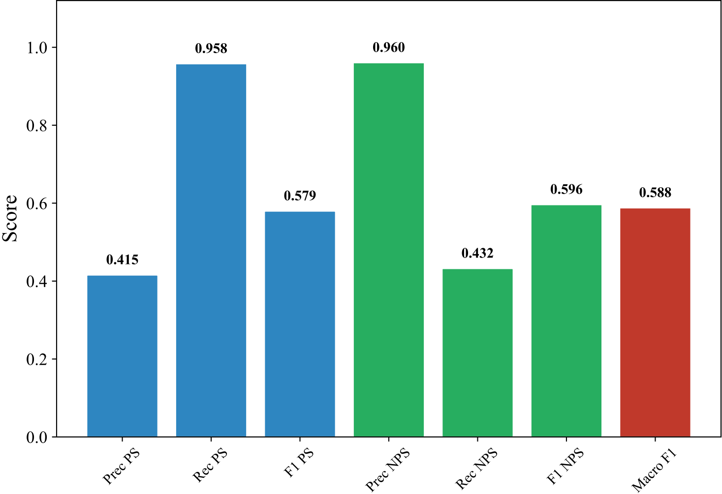
Classification Metrics — DUTCH_MANUAL (intfloat/multilingual-e5-large-instruct, Random_Forest_Optimized)
