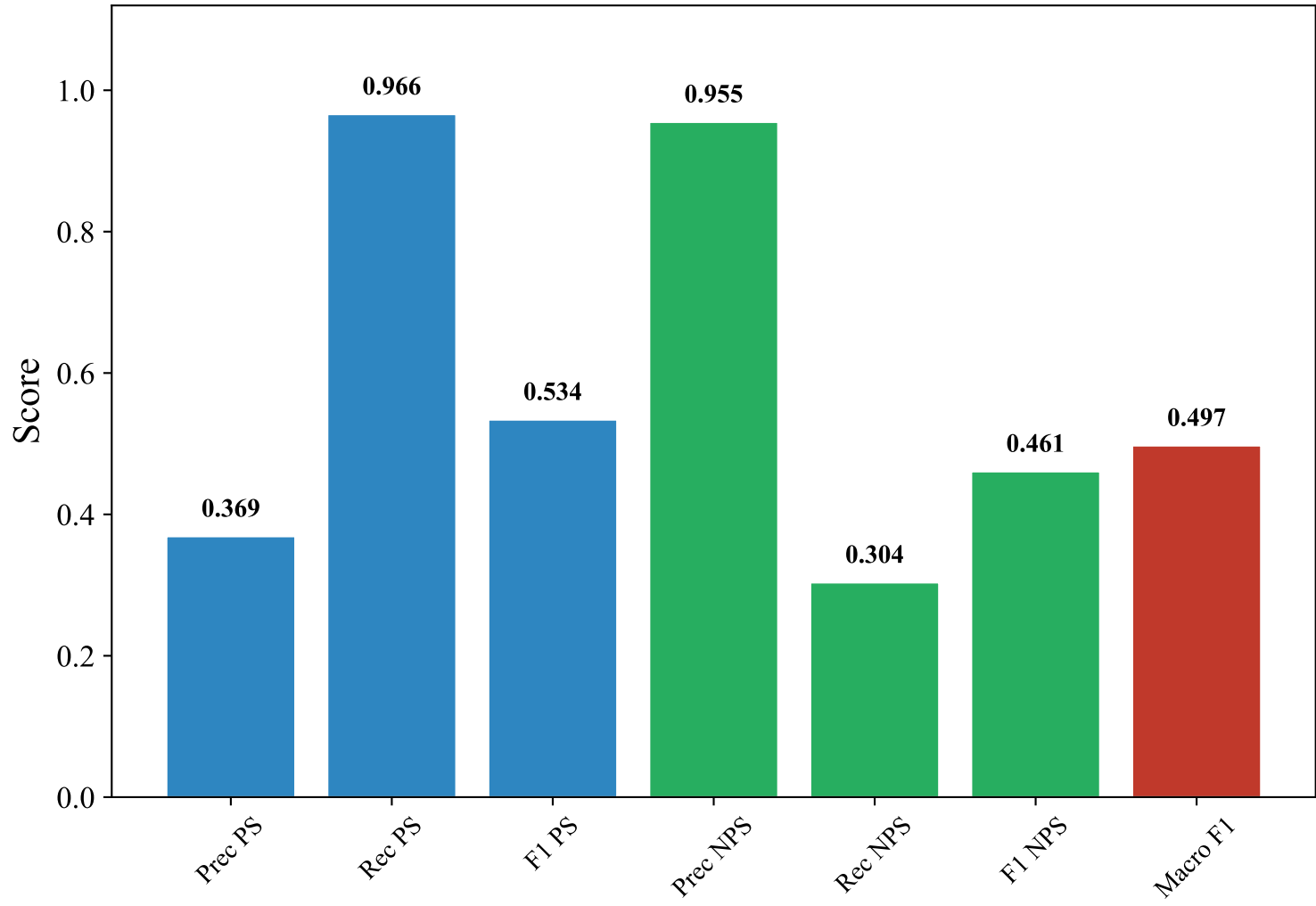
Classification Metrics — DUTCH_MANUAL (upskyy/bge-m3-korean, Random_Forest_Optimized)
