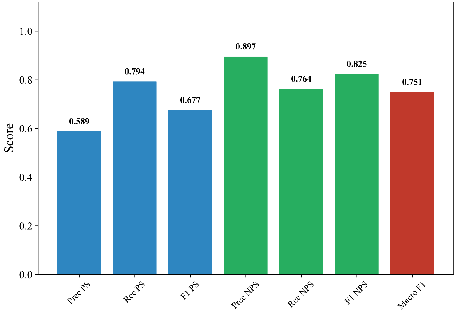
Classification Metrics — ENGLISH_MANUAL (efederici/e5-base-multilingual-4096, Voting_Ensemble)
