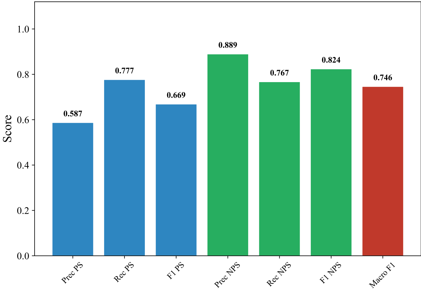
Classification Metrics — ENGLISH_MANUAL (efederici/e5-base-multilingual-4096, XGBoost)
