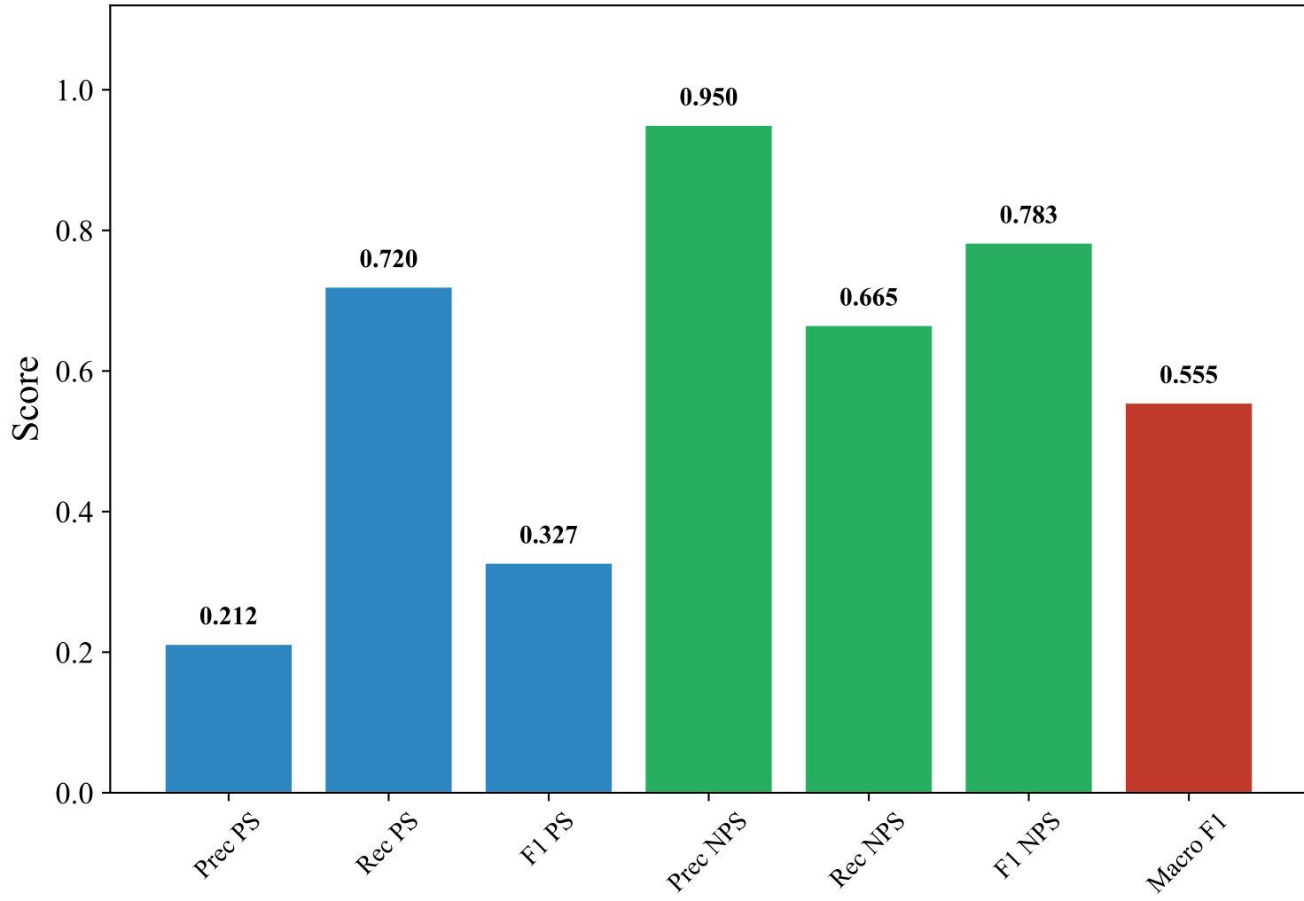
Classification Metrics — GERMAN_MANUAL (efederici/e5-base-multilingual-4096, Random_Forest)
