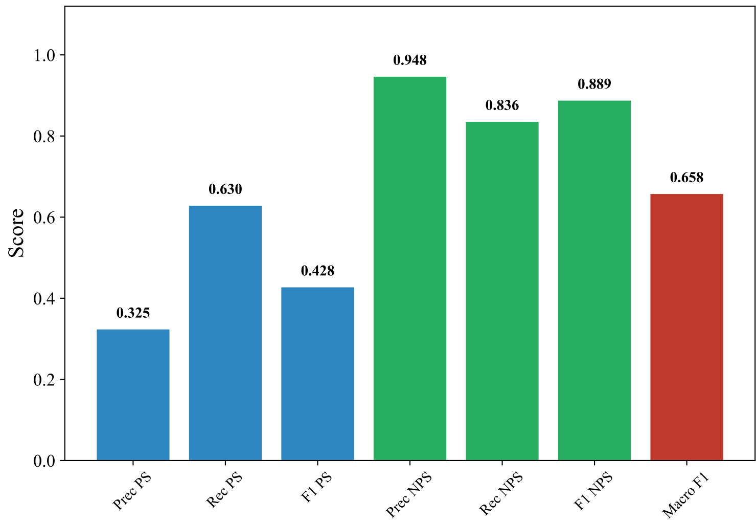
Classification Metrics — GERMAN_MANUAL (efederici/e5-base-multilingual-4096, SVM)
