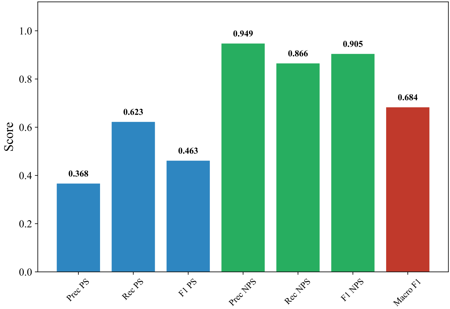
Classification Metrics — GERMAN_MANUAL (efederici/e5-base-multilingual-4096, Voting_Ensemble)
