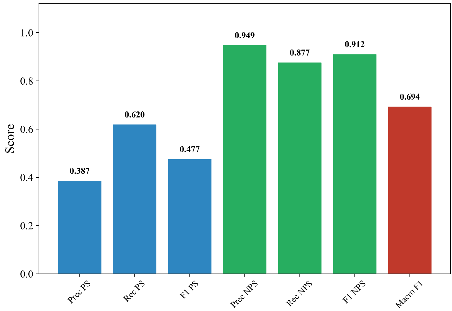
Classification Metrics — GERMAN_MANUAL (efederici/e5-base-multilingual-4096, XGBoost_Optimized)
