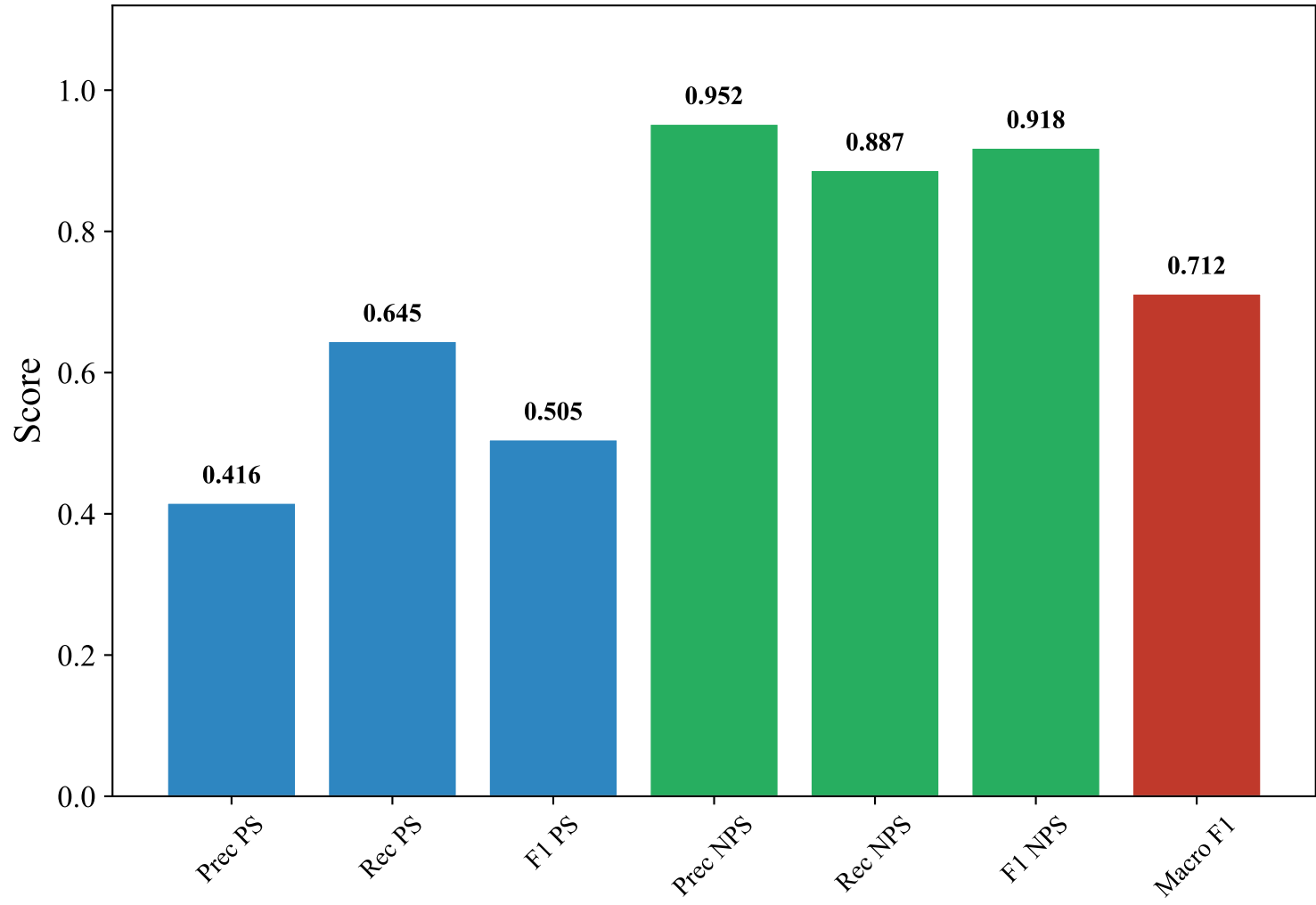
Classification Metrics — GERMAN_MANUAL (intfloat/multilingual-e5-large-instruct, LightGBM)
