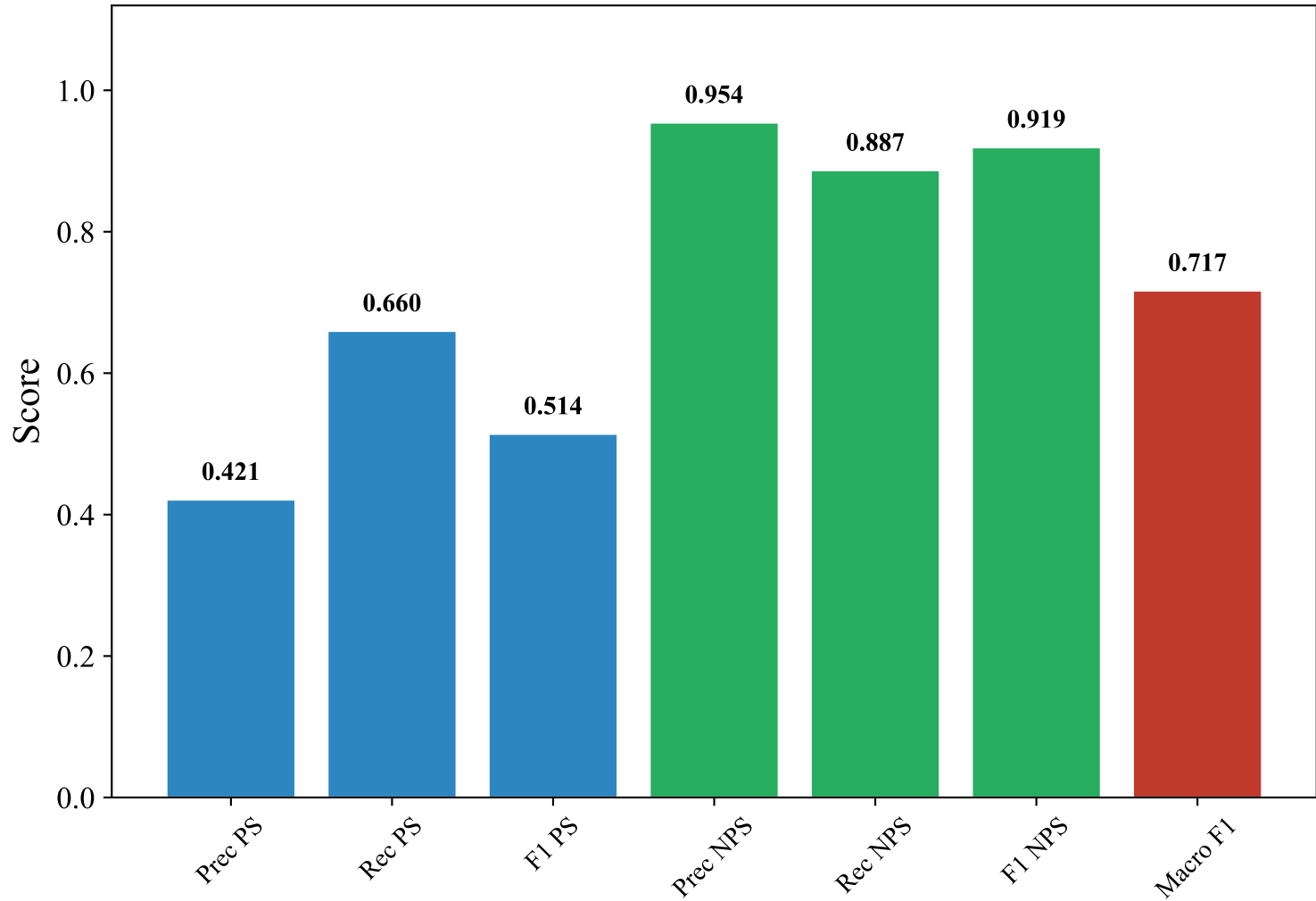
Classification Metrics — GERMAN_MANUAL (intfloat/multilingual-e5-large-instruct, XGBoost)
