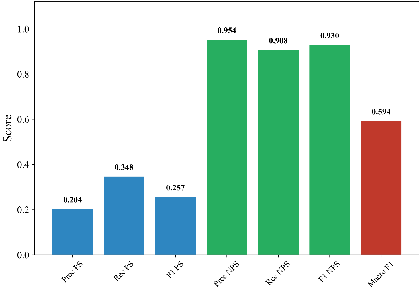
Classification Metrics — SWEDISH_MANUAL (efederici/e5-base-multilingual-4096, LightGBM_Optimized)
