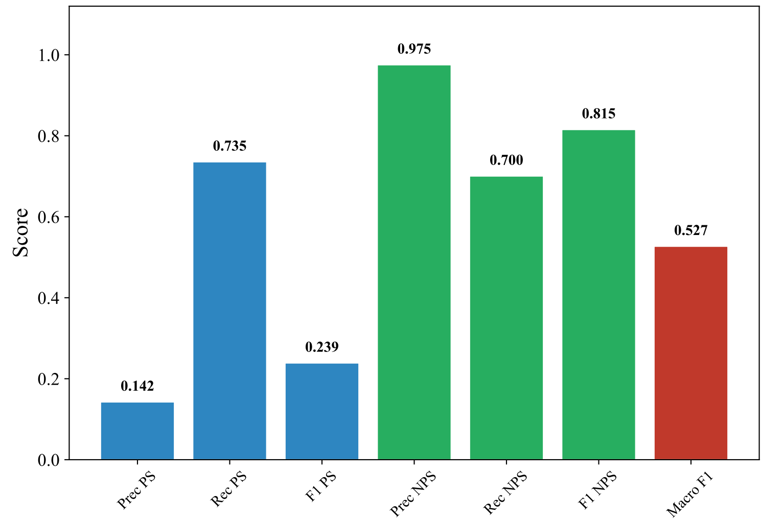
Classification Metrics — SWEDISH_MANUAL (intfloat/multilingual-e5-large-instruct, Random_Forest)
