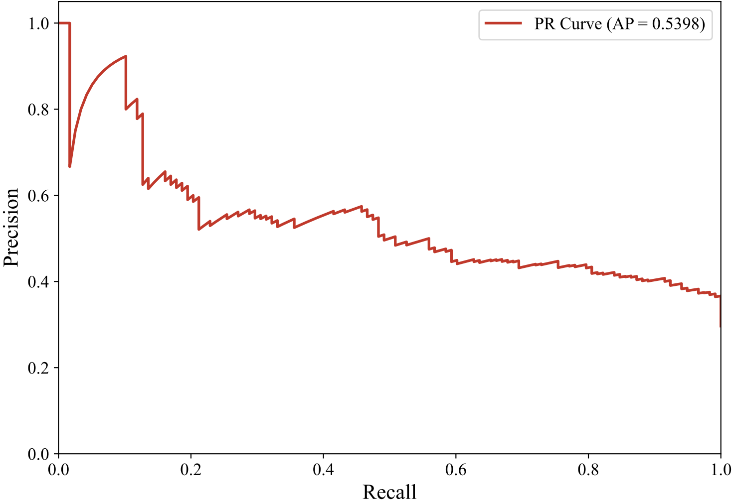
Precision-Recall Curve — DUTCH_MANUAL (efederici/e5-base-multilingual-4096, Random_Forest_Optimized)
