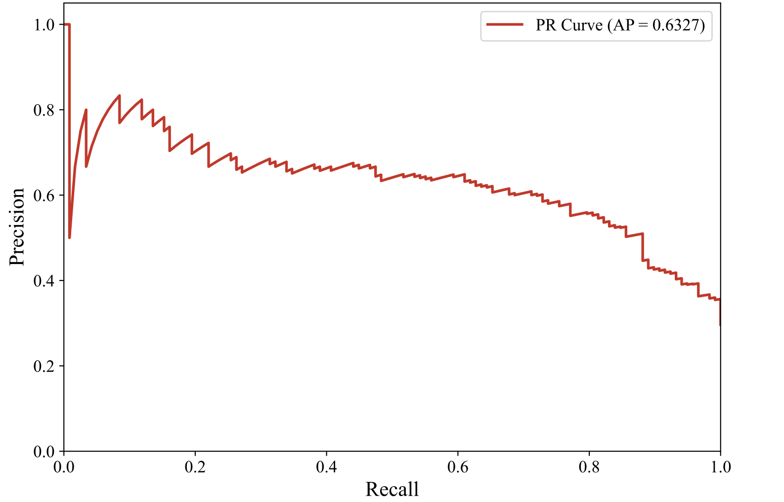
Precision-Recall Curve — DUTCH_MANUAL (intfloat/multilingual-e5-large-instruct, LightGBM)
