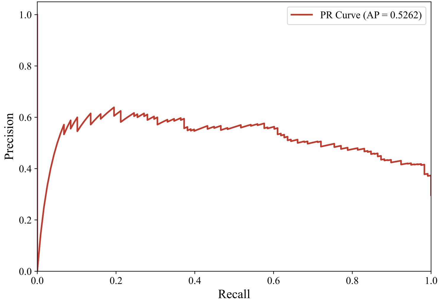
Precision-Recall Curve — DUTCH_MANUAL (intfloat/multilingual-e5-large-instruct, Random_Forest)
