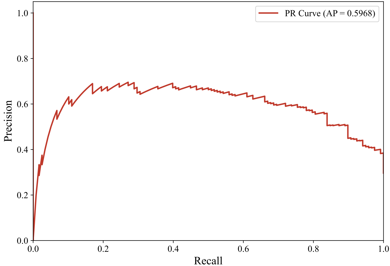
Precision-Recall Curve — DUTCH_MANUAL (intfloat/multilingual-e5-large-instruct, Voting_Ensemble)
