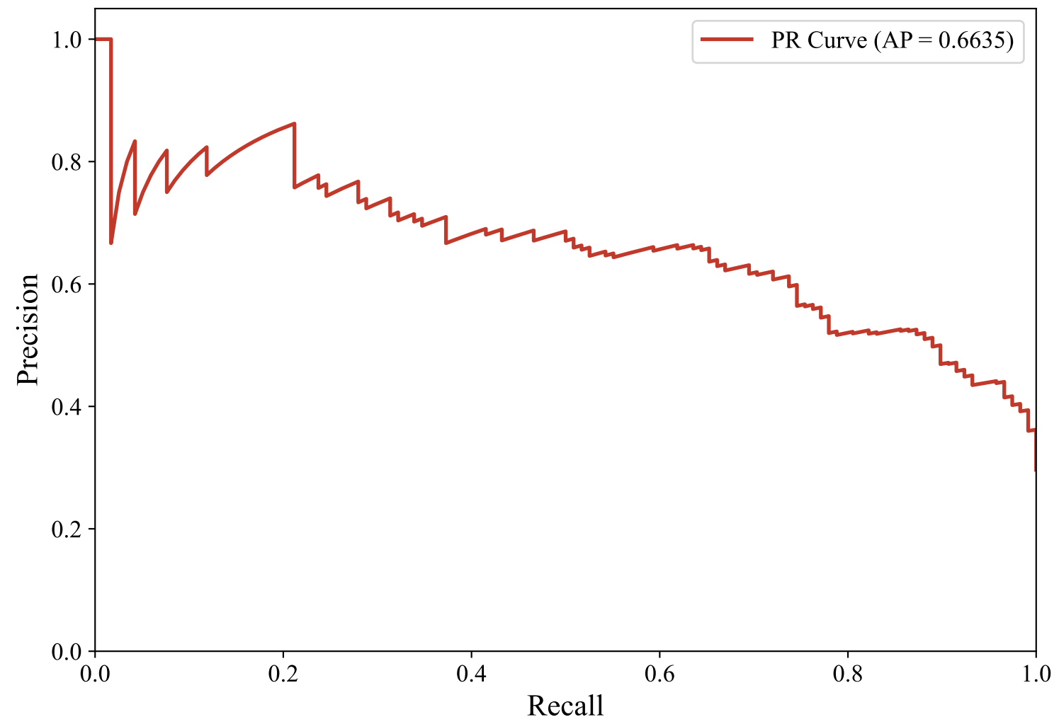
Precision-Recall Curve — DUTCH_MANUAL (intfloat/multilingual-e5-large-instruct, XGBoost)
