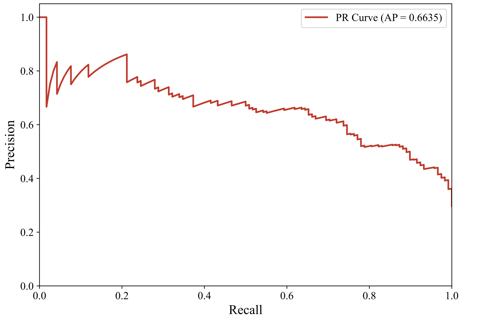
Precision-Recall Curve — DUTCH_MANUAL (intfloat/multilingual-e5-large-instruct, XGBoost_Optimized)
