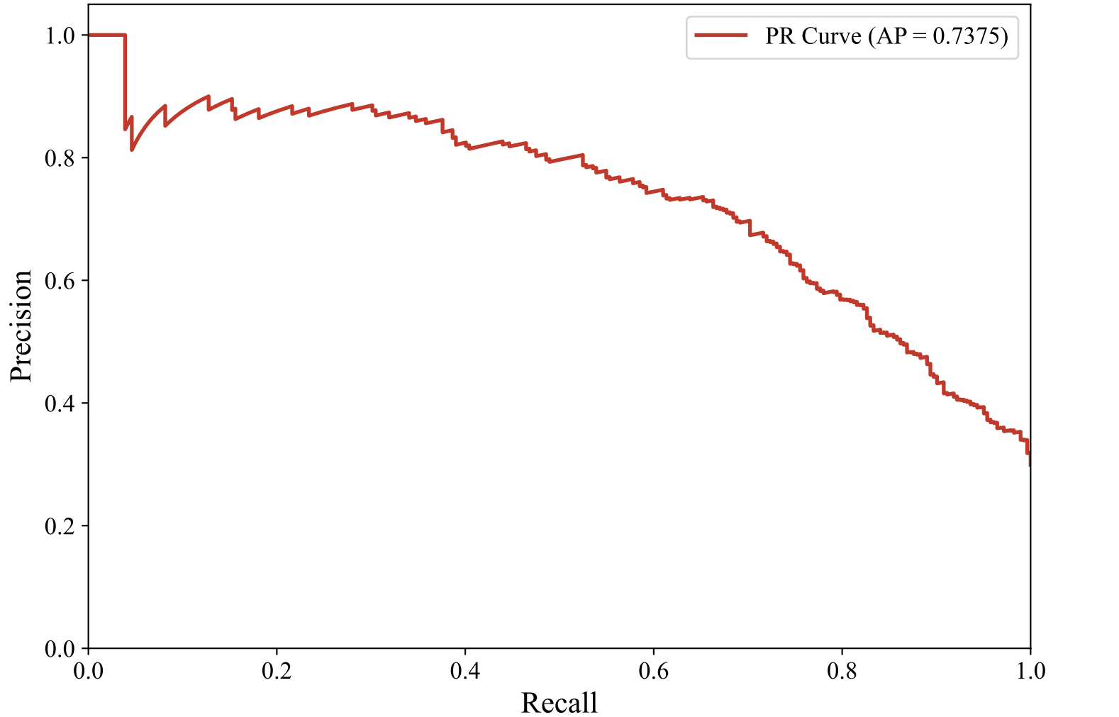
Precision-Recall Curve — ENGLISH_MANUAL (efederici/e5-base-multilingual-4096, XGBoost_Optimized)
