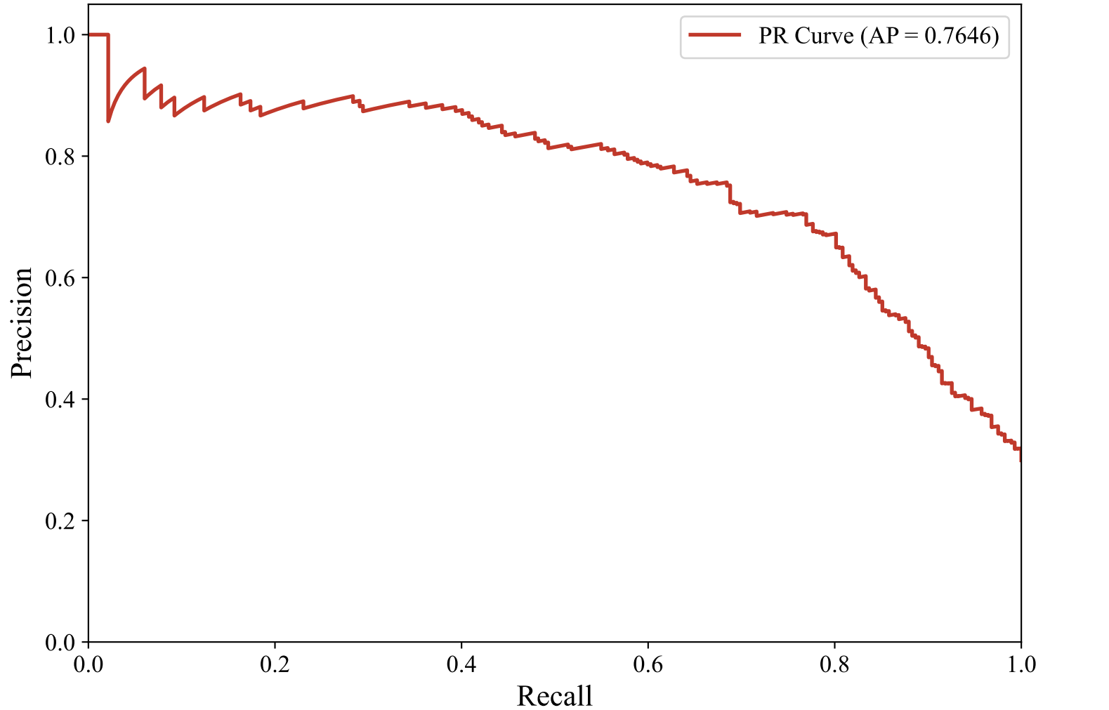
Precision-Recall Curve — ENGLISH_MANUAL (intfloat/multilingual-e5-large-instruct, LightGBM)
