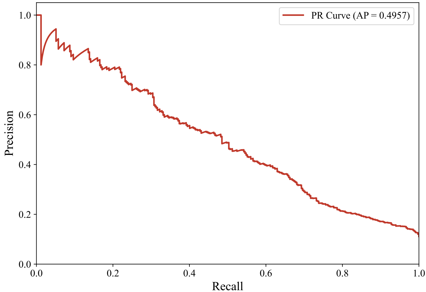
Precision-Recall Curve — GERMAN_MANUAL (efederici/e5-base-multilingual-4096, XGBoost)
