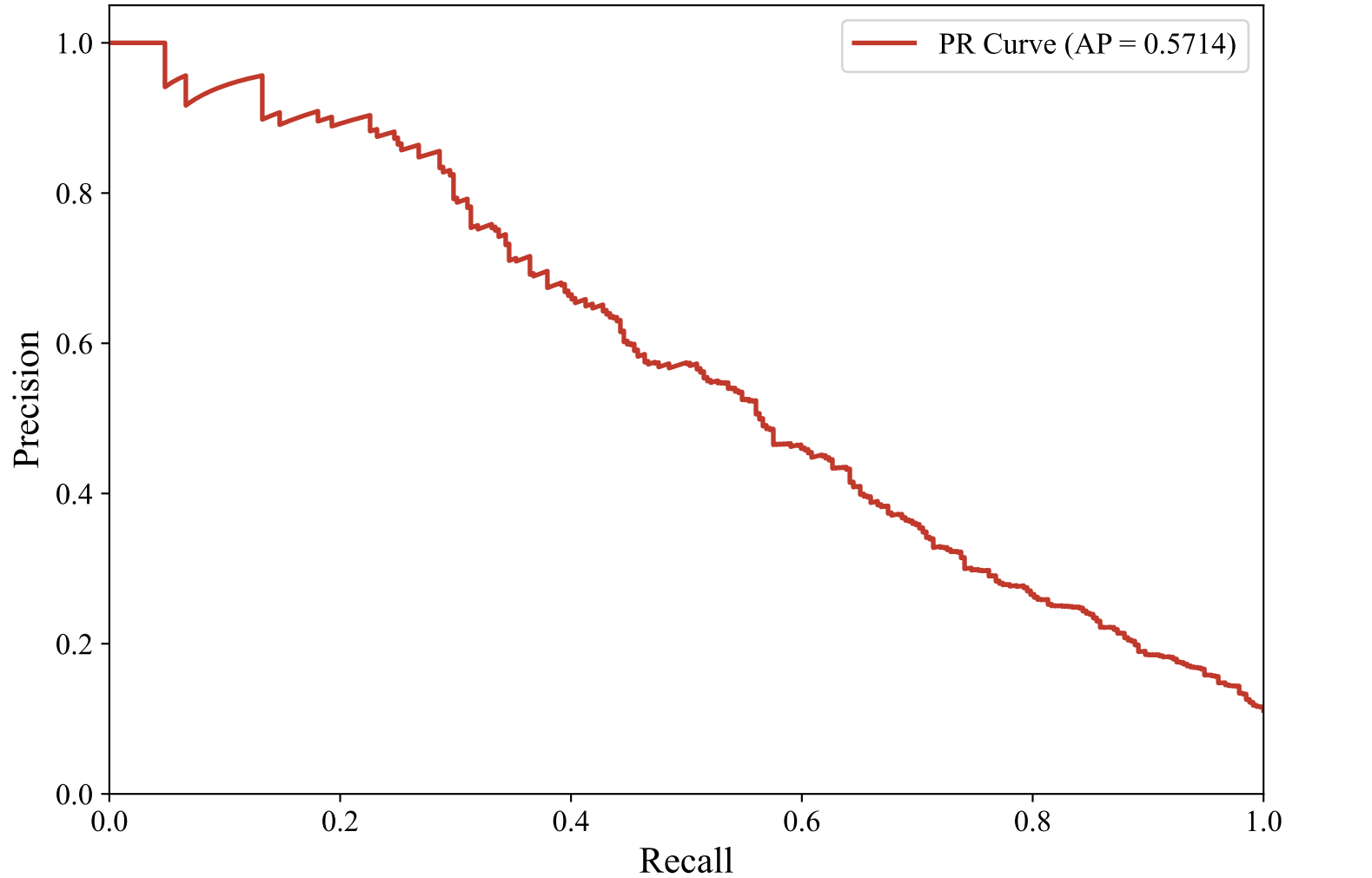
Precision-Recall Curve — GERMAN_MANUAL (intfloat/multilingual-e5-large-instruct, LightGBM)
