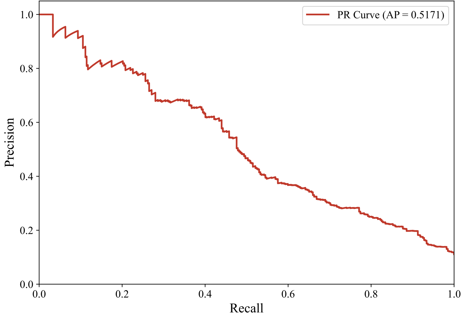
Precision-Recall Curve — GERMAN_MANUAL (intfloat/multilingual-e5-large-instruct, Random_Forest_Optimized)
