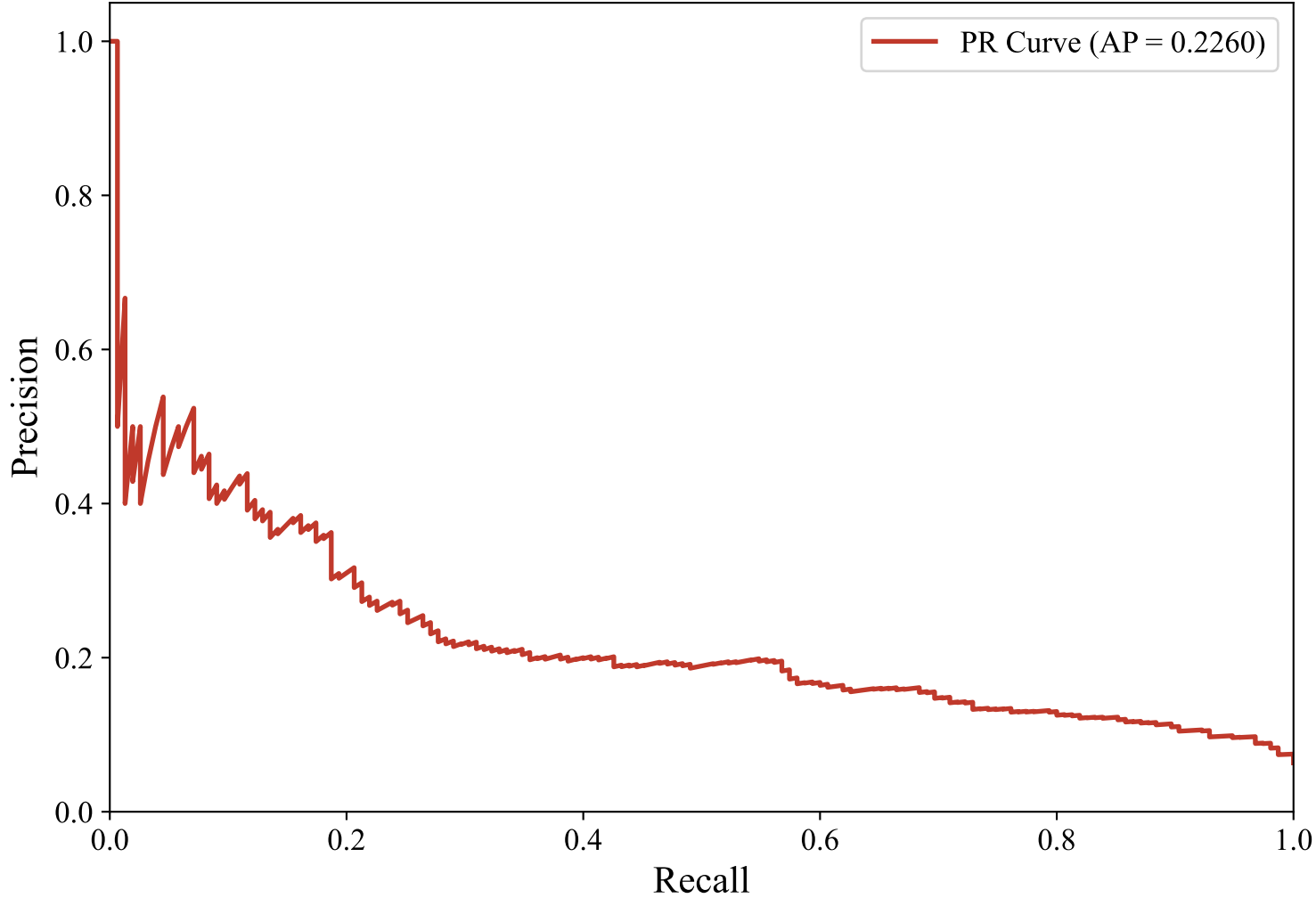
Precision-Recall Curve — SWEDISH_MANUAL (efederici/e5-base-multilingual-4096, LightGBM_Optimized)
