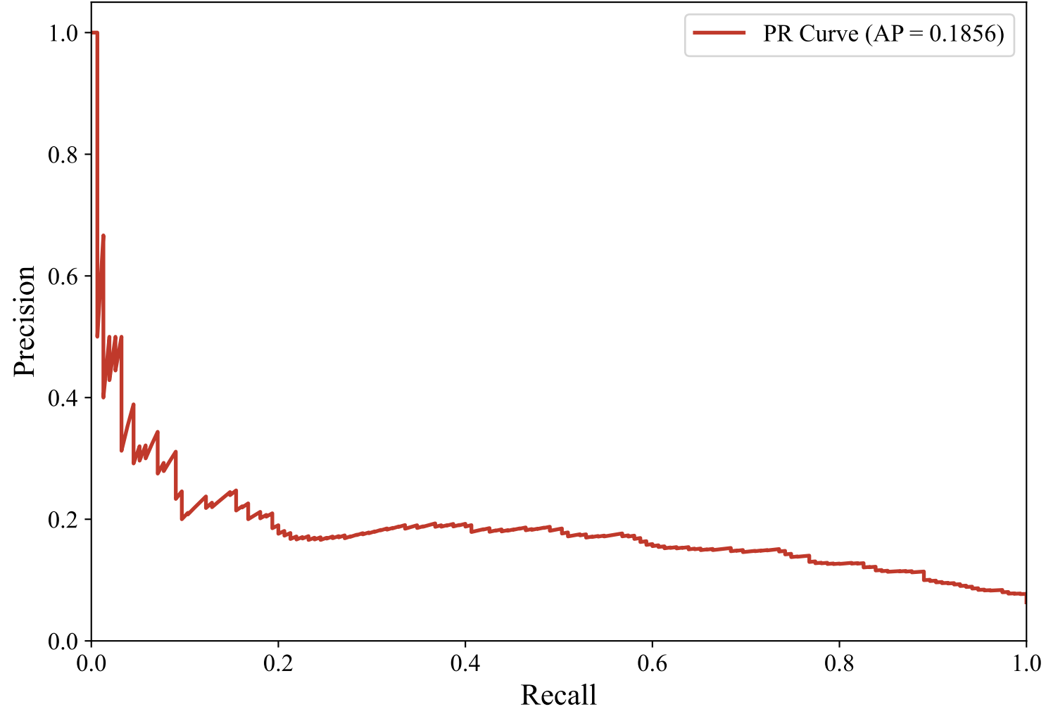
Precision-Recall Curve — SWEDISH_MANUAL (efederici/e5-base-multilingual-4096, Random_Forest_Optimized)
