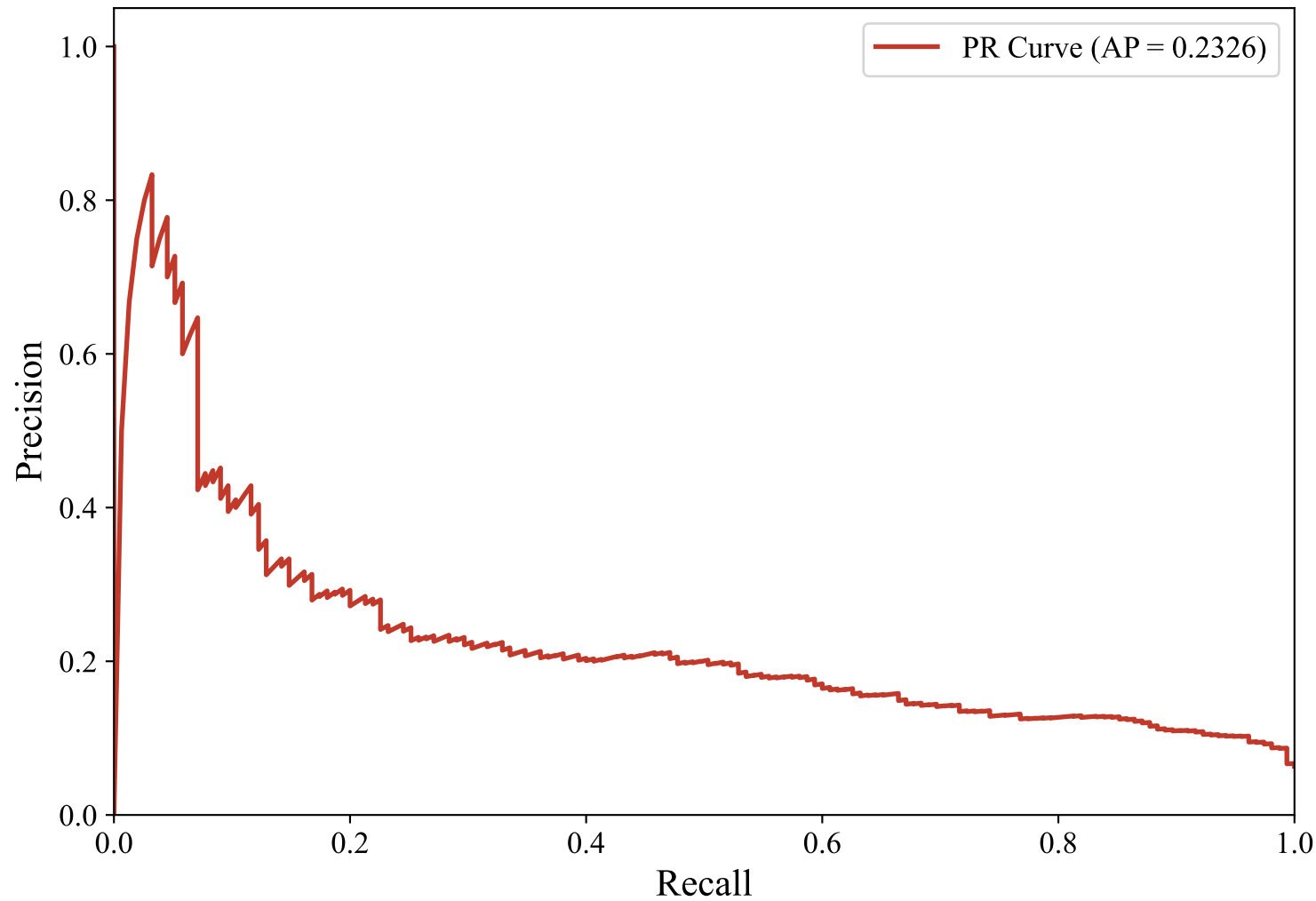
Precision-Recall Curve — SWEDISH_MANUAL (efederici/e5-base-multilingual-4096, XGBoost)
