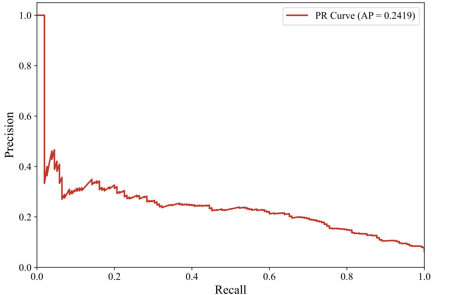
Precision-Recall Curve — SWEDISH_MANUAL (intfloat/multilingual-e5-large-instruct, XGBoost_Optimized)
