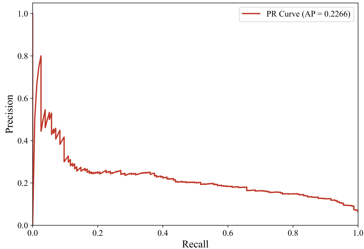
Precision-Recall Curve — SWEDISH_MANUAL (upskyy/bge-m3-korean, Voting_Ensemble)
