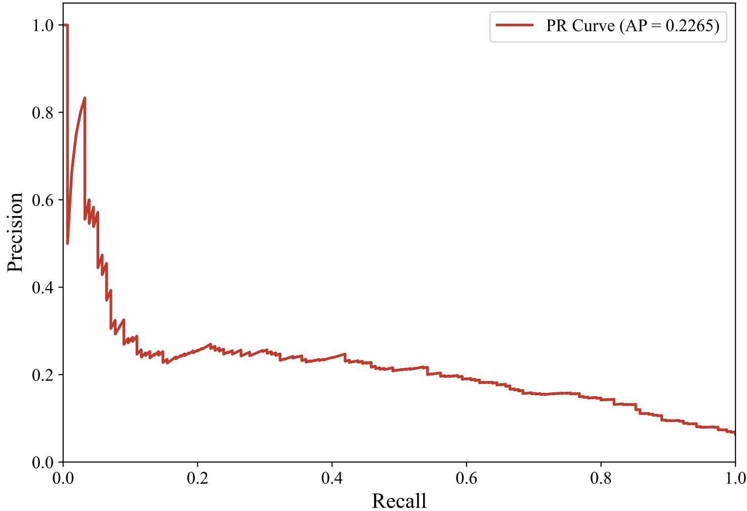
Precision-Recall Curve — SWEDISH_MANUAL (upskyy/bge-m3-korean, XGBoost_Optimized)
