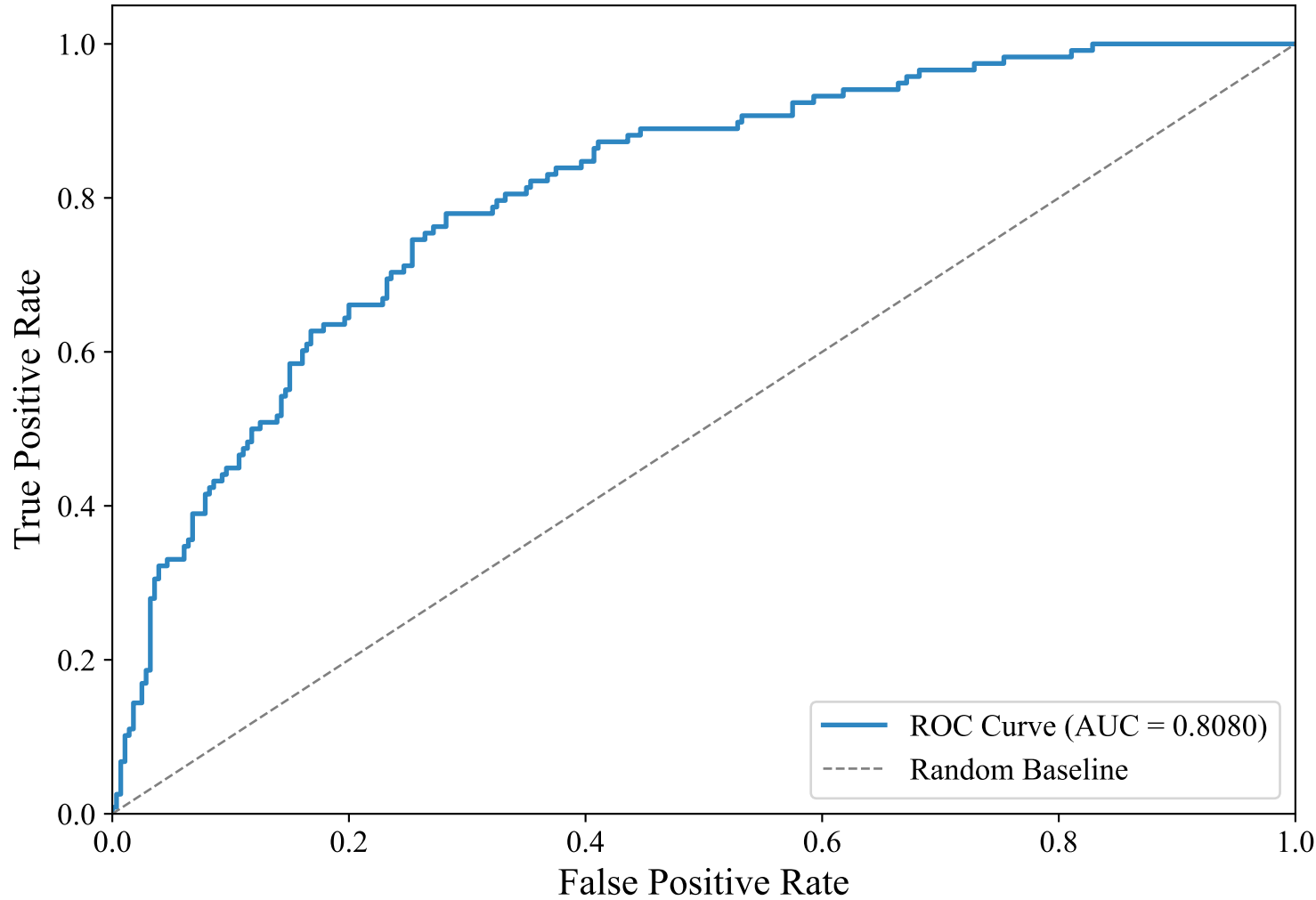
ROC Curve — DUTCH_MANUAL (efederici/e5-base-multilingual-4096, LightGBM_Optimized)
