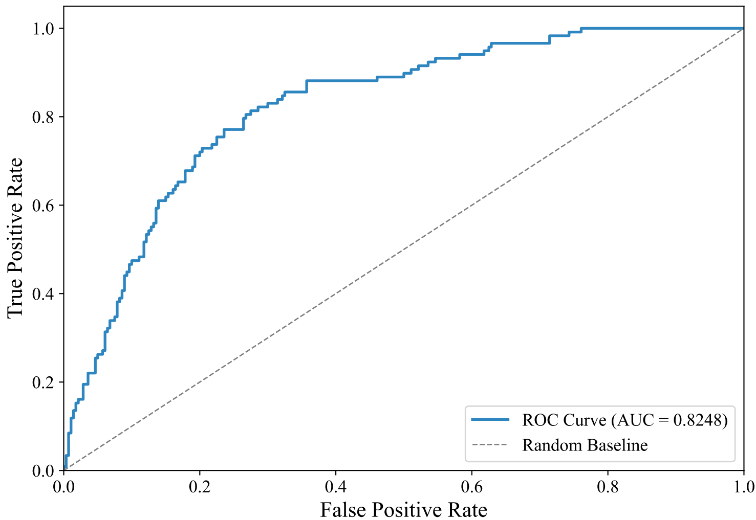
ROC Curve — DUTCH_MANUAL (intfloat/multilingual-e5-large-instruct, LightGBM)
