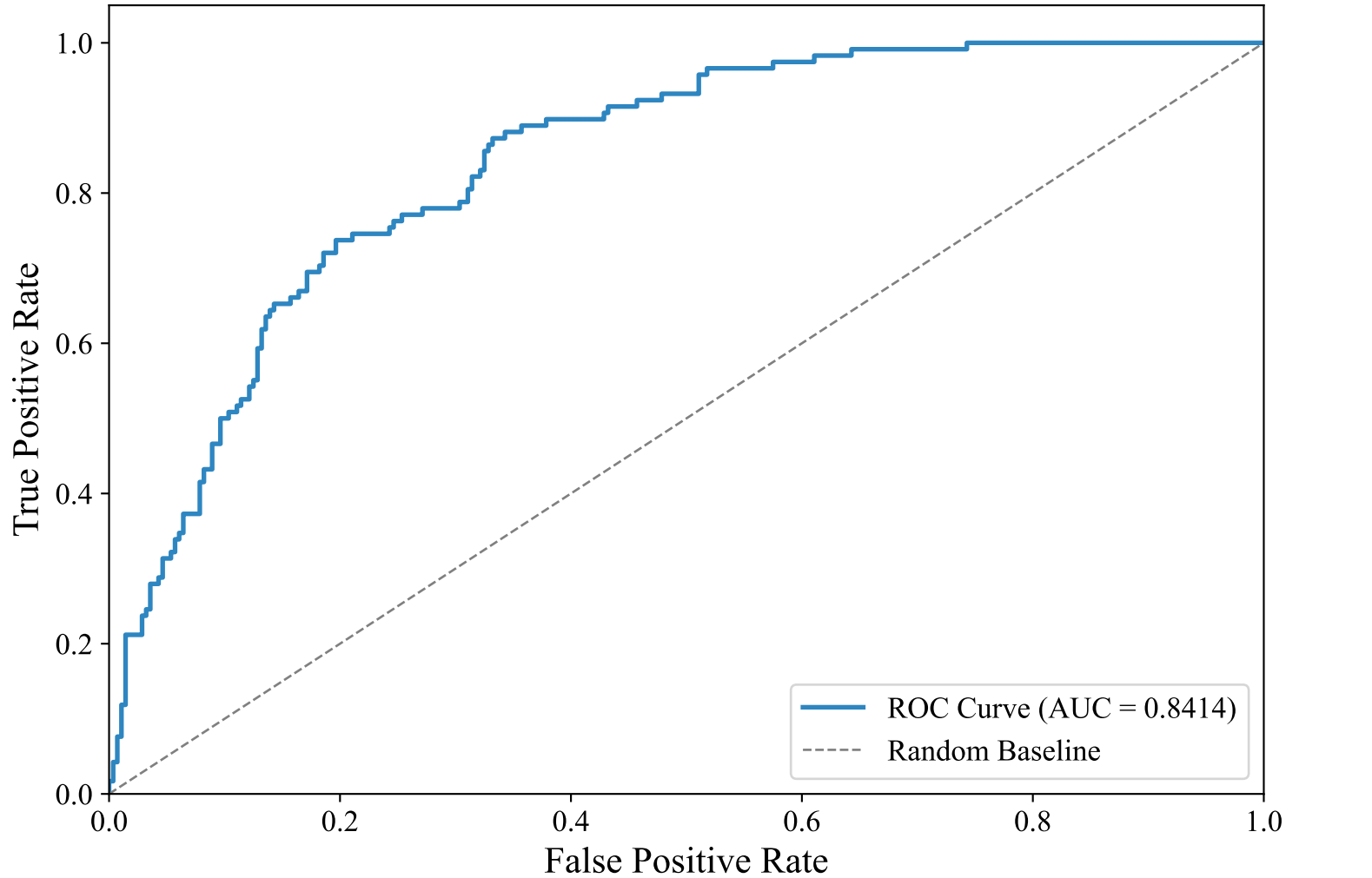
ROC Curve — DUTCH_MANUAL (intfloat/multilingual-e5-large-instruct, XGBoost)
