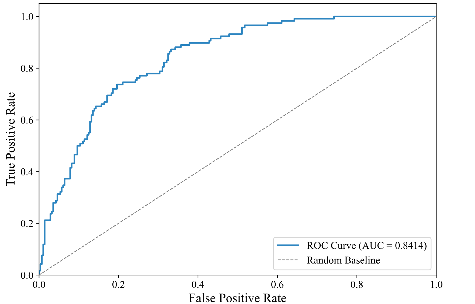
ROC Curve — DUTCH_MANUAL (intfloat/multilingual-e5-large-instruct, XGBoost_Optimized)
