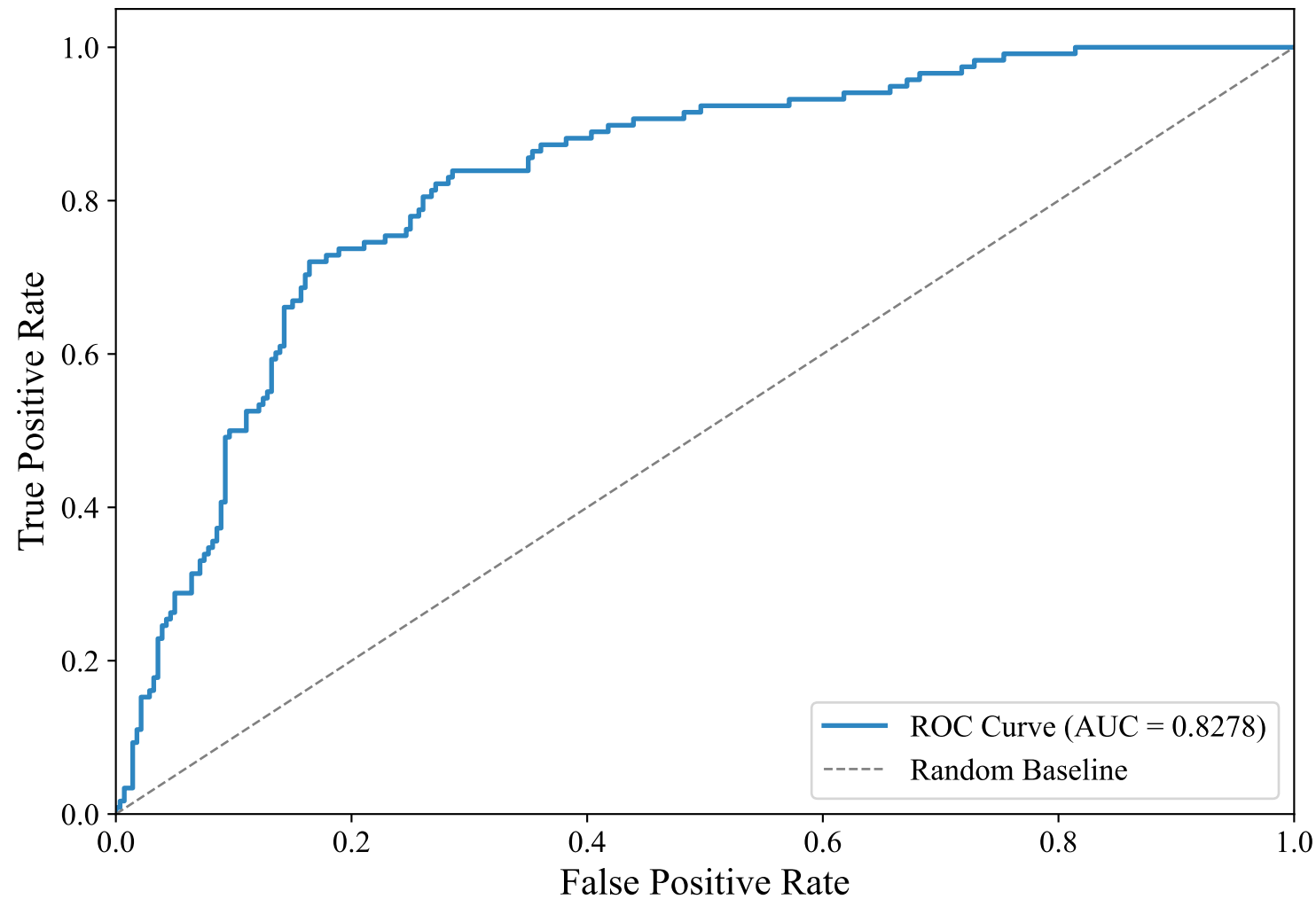
ROC Curve — DUTCH_MANUAL (upskyy/bge-m3-korean, LightGBM)
