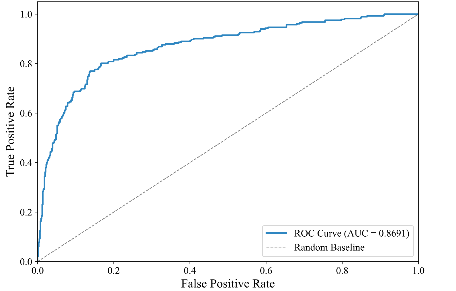
ROC Curve — ENGLISH_MANUAL (intfloat/multilingual-e5-large-instruct, LightGBM_Optimized)
