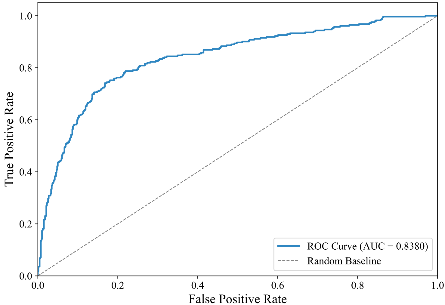
ROC Curve — ENGLISH_MANUAL (intfloat/multilingual-e5-large-instruct, Random_Forest_Optimized)
