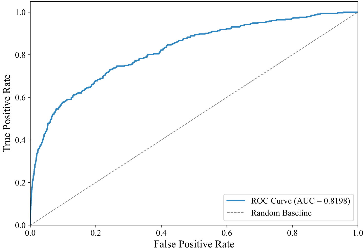
ROC Curve — GERMAN_MANUAL (efederici/e5-base-multilingual-4096, LightGBM)
