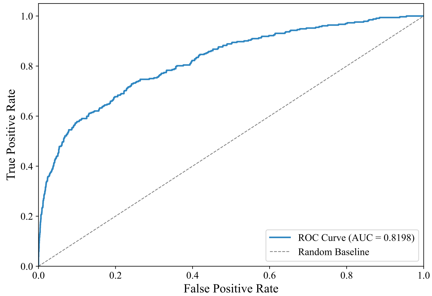
ROC Curve — GERMAN_MANUAL (efederici/e5-base-multilingual-4096, LightGBM_Optimized)
