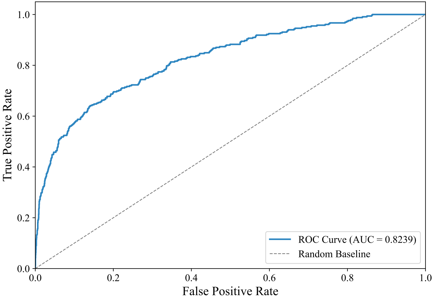
ROC Curve — GERMAN_MANUAL (efederici/e5-base-multilingual-4096, Voting_Ensemble)
