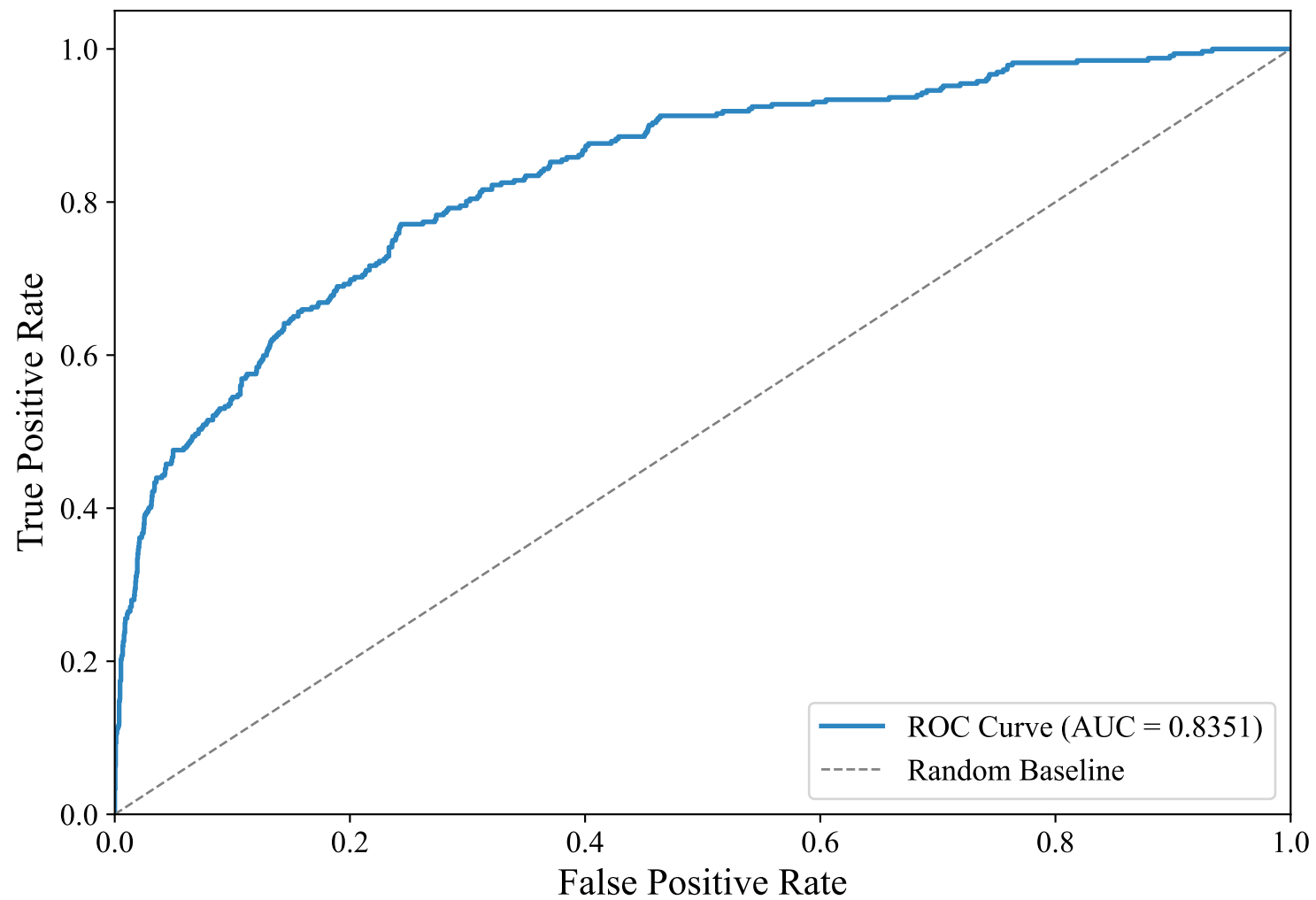
ROC Curve — GERMAN_MANUAL (intfloat/multilingual-e5-large-instruct, Random_Forest)
