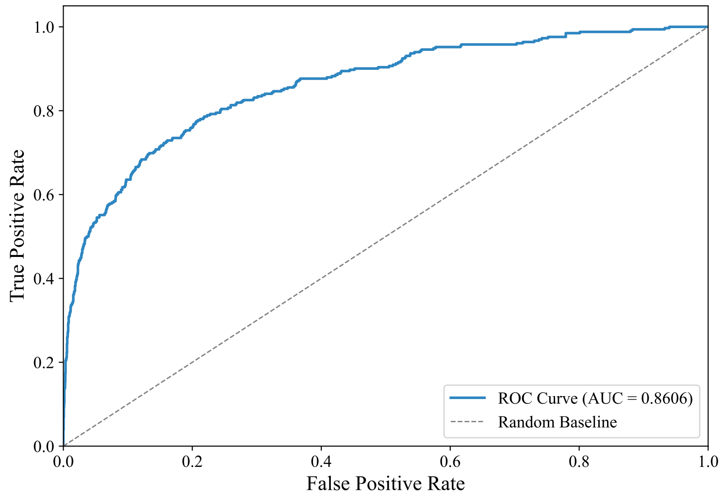
ROC Curve — GERMAN_MANUAL (intfloat/multilingual-e5-large-instruct, Voting_Ensemble)
