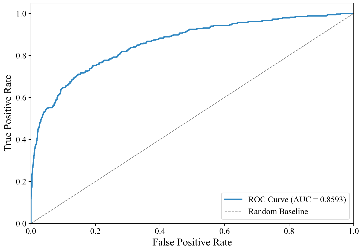
ROC Curve — GERMAN_MANUAL (intfloat/multilingual-e5-large-instruct, XGBoost)
