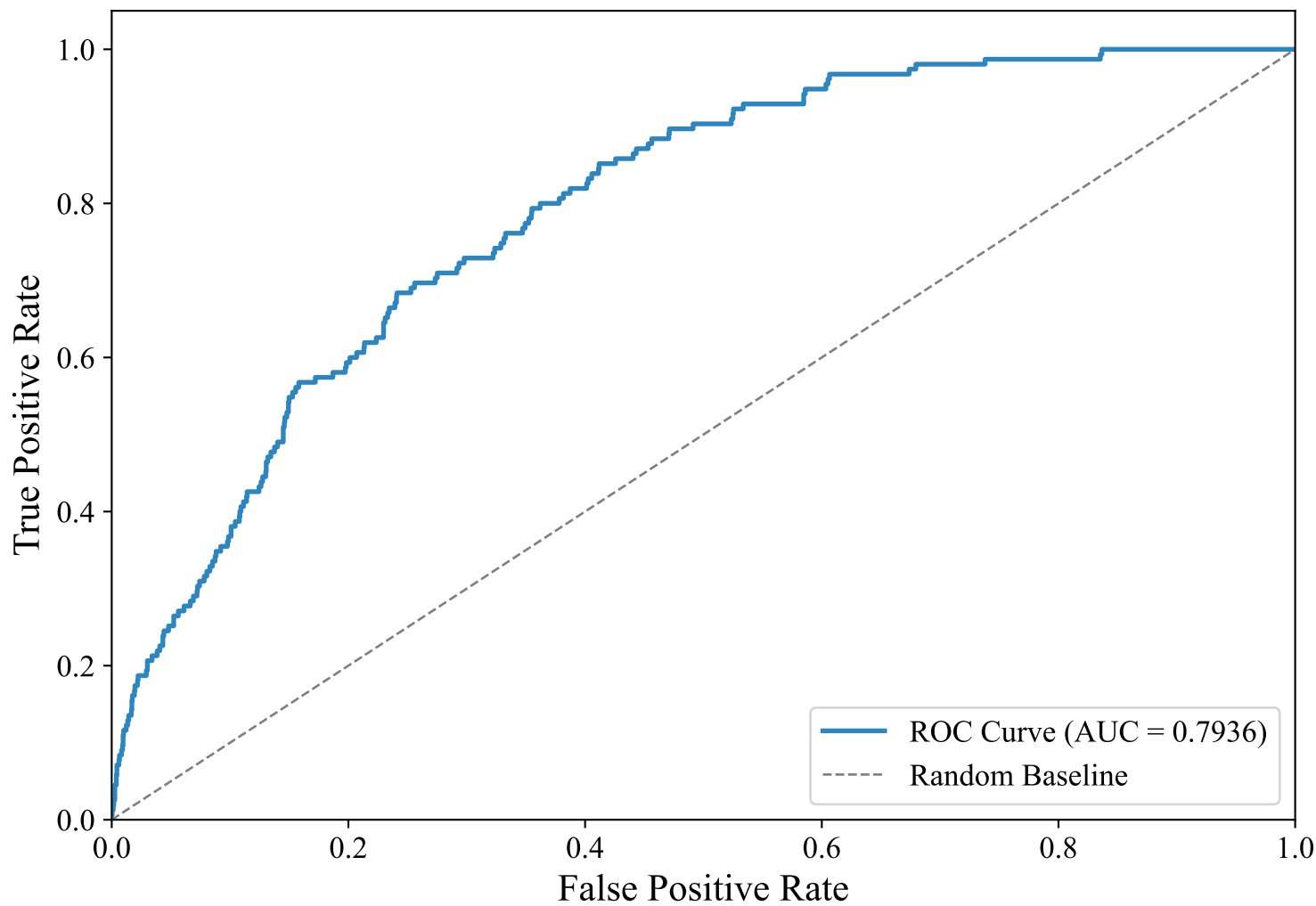
ROC Curve — SWEDISH_MANUAL (efederici/e5-base-multilingual-4096, LightGBM)
