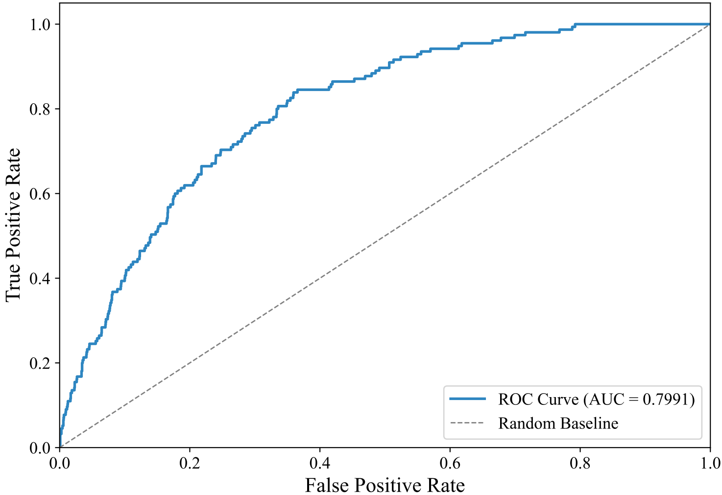
ROC Curve — SWEDISH_MANUAL (efederici/e5-base-multilingual-4096, Voting_Ensemble)
