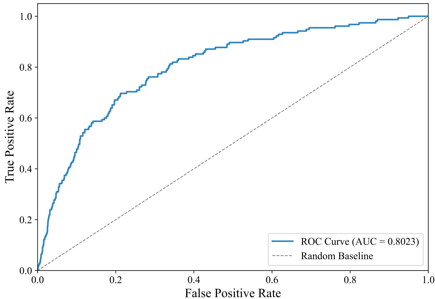
ROC Curve — SWEDISH_MANUAL (intfloat/multilingual-e5-large-instruct, LightGBM)
