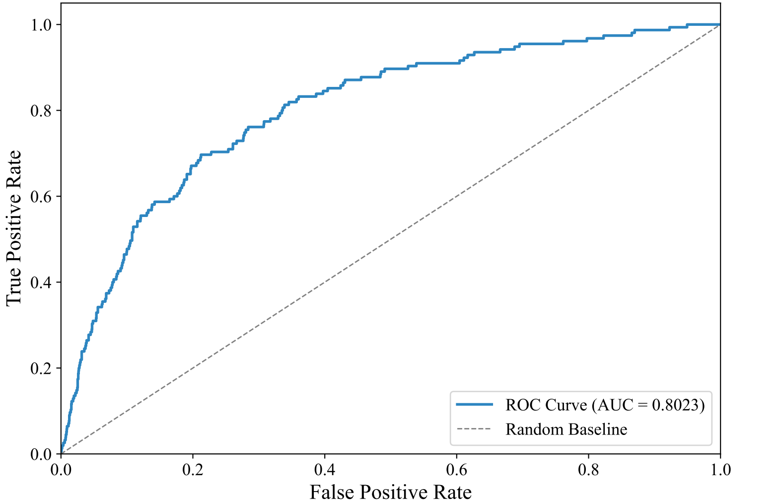
ROC Curve — SWEDISH_MANUAL (intfloat/multilingual-e5-large-instruct, LightGBM_Optimized)
